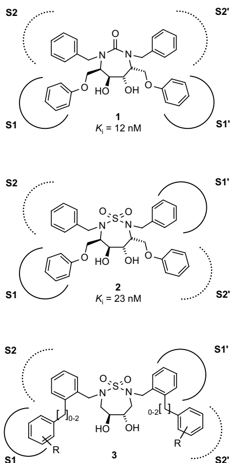
Figure 1. Structure of a cyclic urea inhibitor 1 with symmetric binding to HIV-1 protease and a cyclic sulfamide inhibitor 2 with nonsymmetric binding. The generic structure 3 and the proposed nonsymmetric binding to HIV-1 protease.
