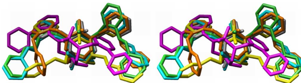
Figure 2. Results from the Monte Carlo conformational search. Depicted are the low energy conformations of 9 (gray), 10 (green), 11 (cyan), 12 (orange), and 13 (magenta), the X-ray crystal structure of 2 (yellow) is included for comparison. The molecular graphics image was produced using the UCSF Chimera. 32
