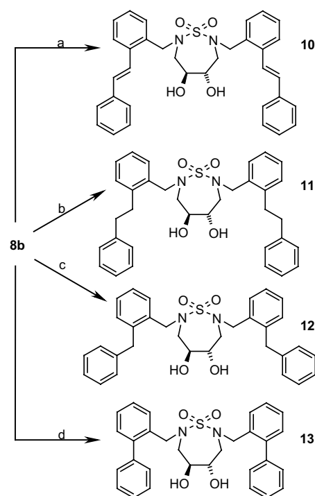
Scheme 2. Reagents and conditions: (a) i. styrene, DIEA, \text{Pd}(\text{OAc})_2 , \text{PPh}_3 , DMF, \text{H}_2\text{O} , microwaves 150^\circ\text{C} , 20 min, ii. \text{HCl} /ether and methanol; (b) i. styrene, DIEA, \text{Pd}(\text{OAc})_2 , \text{PPh}_3 , DMF, \text{H}_2\text{O} , microwaves 150^\circ\text{C} , 20 min, ii. \text{H}_2 , \text{Pd/C} , ethyl acetate, iii. \text{HCl} /ether and methanol; (c) i. benzyl zinc, \text{PdCl}_2 , DPPF, THF under \text{N}_2 , 80^\circ\text{C} , 88 h, ii. \text{HCl} /ether and methanol; (d) i. phenyl boronic acid, \text{Pd}(\text{OAc})_2 , \text{PPh}_3 , \text{Na}_2\text{CO}_3 , DME, ethanol, microwaves 150^\circ\text{C} , 5 min, ii. \text{HCl} /ether and methanol.
