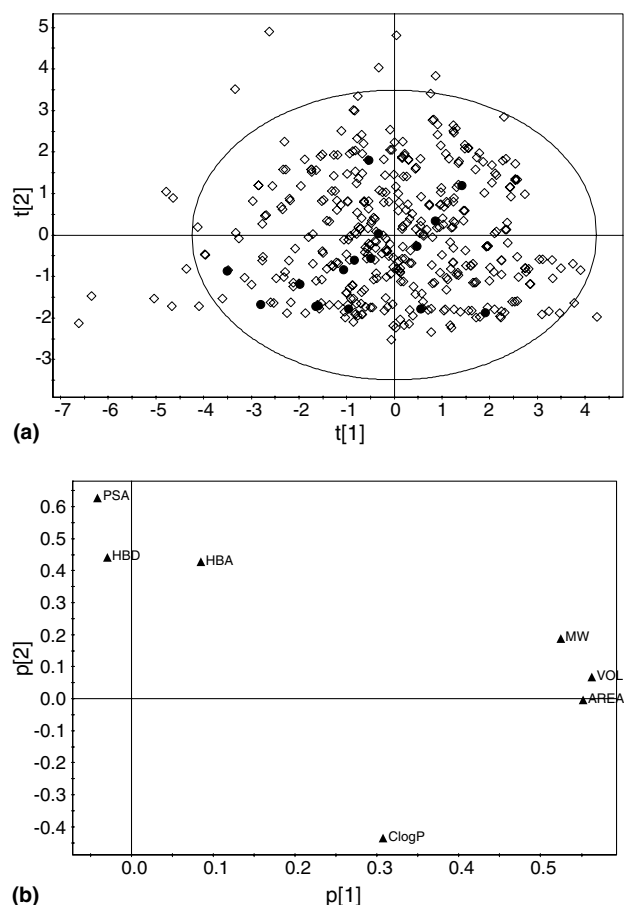
Figure 3. Results from the principal component analysis (PCA) for the selected boronic acids and esters. In score plot (a), the building blocks used are depicted (black dots) among the commercially available building blocks (open diamond). Analyzing the loading plot (b), a preference for lipophilic compounds with low molecular weight can be seen, which corresponds to our design criterion.
