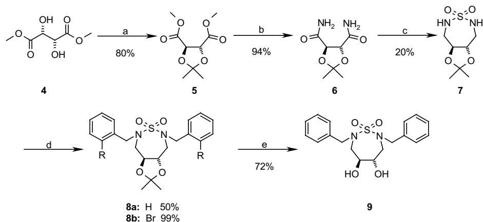
Scheme 1. Reagents and conditions: (a) 2,2-dimethoxypropane and DL-10-camphorsulfonic acid in acetone; (b) \text{NH}_3 /methanol; (c) i. \text{LiAlH}_4 in THF, 80^\circ\text{C} , ii. \text{NH}_2\text{SO}_2\text{NH}_2 , \text{Et}_3\text{N} , toluene, 120^\circ\text{C} ; (d) for 8a benzyl bromide, DMF, \text{K}_2\text{CO}_3 and for 8b 2-bromobenzyl bromide, DMF, \text{K}_2\text{CO}_3 ; (e) \text{HCl} /ether and methanol.
